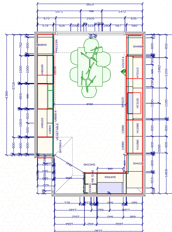
Detailed Layout & Plan
